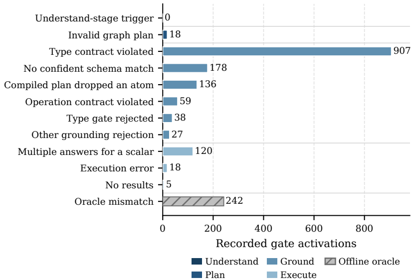
(a) Stage-specific gate activity
