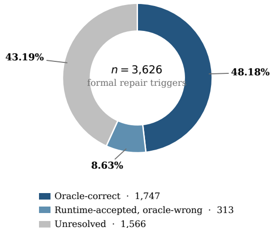
(b) Outcome after bounded repair
